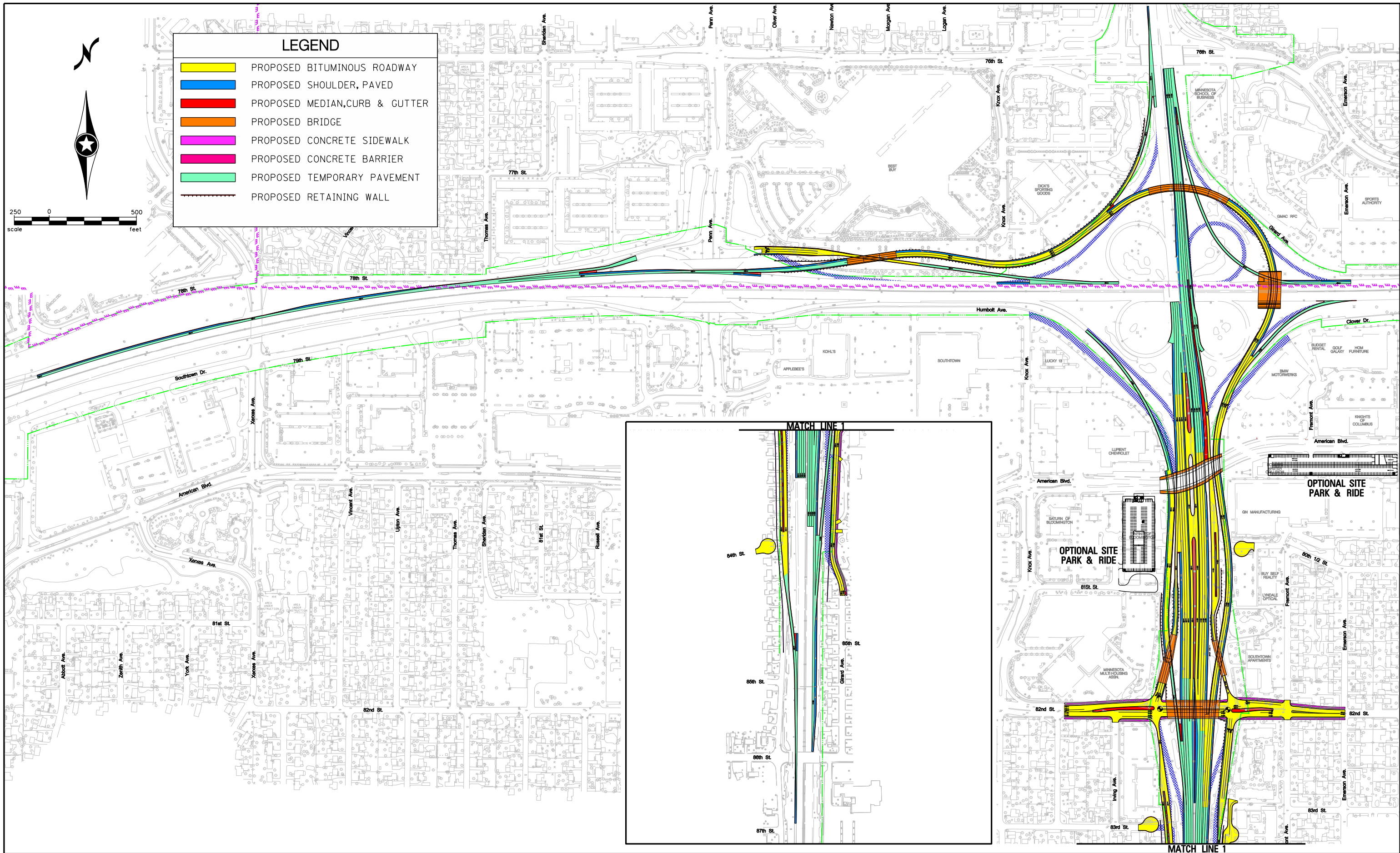
TURBINE-PHASE 1 : BRT AT AMERICAN BLVD. I-494 /35W INTERCHANGE PRELIMINARY DESIGN PROJECT S.P. 2785-350
