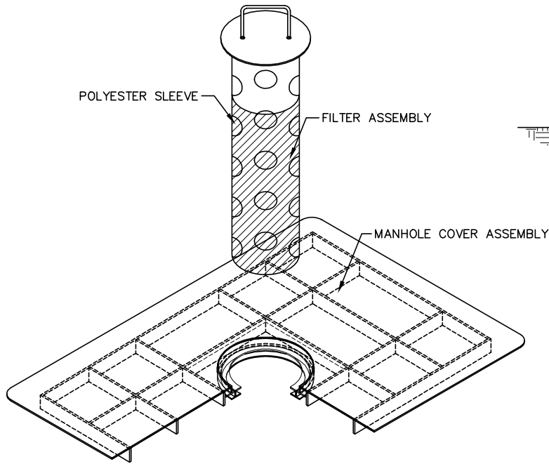
602 - INLET PROTECTION, MANHOLE COVER ASSEMBLY 602 - Wimco (MH).dwg 5/2015
