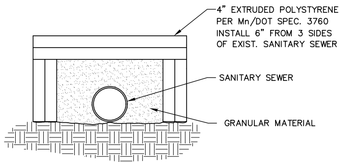
411 - SANITARY SEWER INSULATION DETAIL 411 - San Insulation.dwg 6/2015
