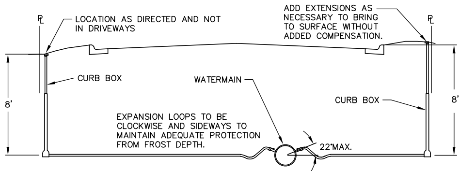
306 - TYPICAL WATER SERVICE 306 - Wat Serv.dwg 6/2015
