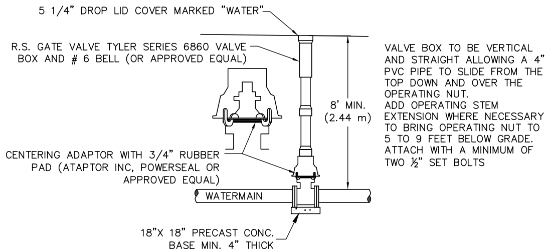
302 - TYPICAL VALVE INSTALLATION 302 - Valve (RSGV).dwg 6/2015
