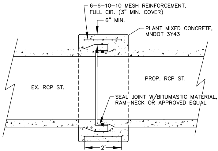
212 - STD CONST. JOINT 212 - STD CONST. JOINT.DWG 6/2016
