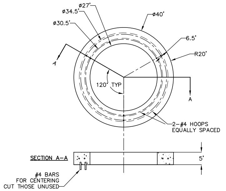
209 - MH ACCESS REDUCER (ADAPT) 209 - MH ACCESS REDUCER (ADAPT).DWG 6/2016
