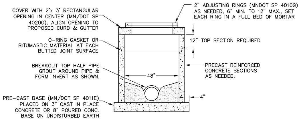
203 - STD MH (CB-MH) 203 - STD MH (CB-MH).DWG 9/2016
