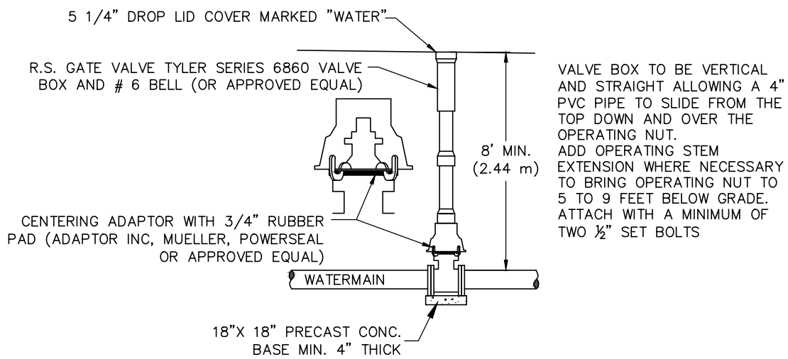
302 - TYPICAL VALVE INSTALLATION 302 - Valve (RSGV).dwg 6/2015
