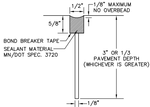
136 - SAW-SEAL (JOINT)
