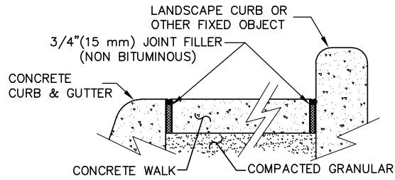
126 - EXPANSION JOINT DETAIL 126 - Typ Expansion Joint.dwg 6/2015
