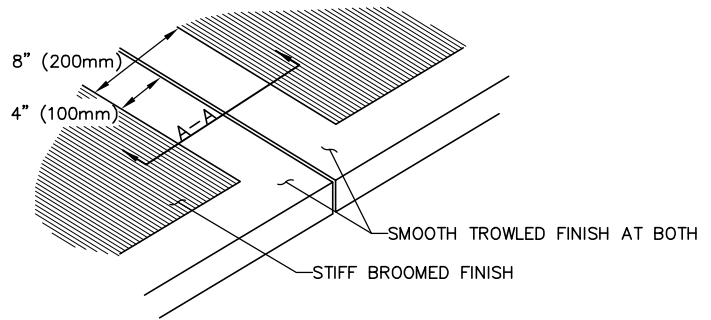
122 - CONC WALK (WITH SIDE REVEAL) 122 - Conc Walk (w-Side Reveal).dwg 5/2015
