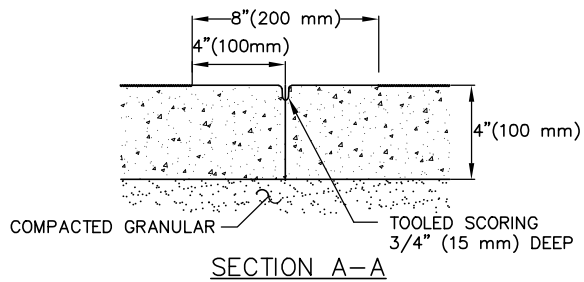
122 - CONC WALK (WITH SIDE REVEAL) 122 - Conc Walk (w-Side Reveal).dwg 5/2015
