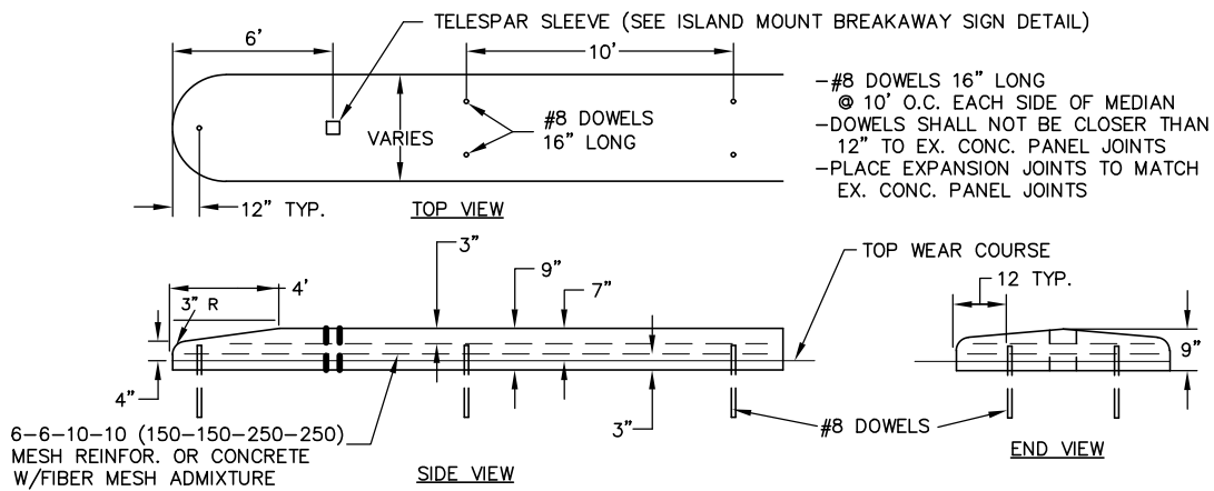
114 - 9" SURFACE CONCRETE MEDIAN 114 - 9 Conc Surf Median.dwg 9/2016
