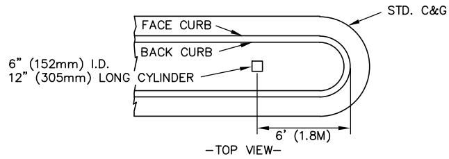
112 - STANDARD CURB & GUTTER MEDIAN 112 - Median Detail (Round Nose).dwg 6/2015
