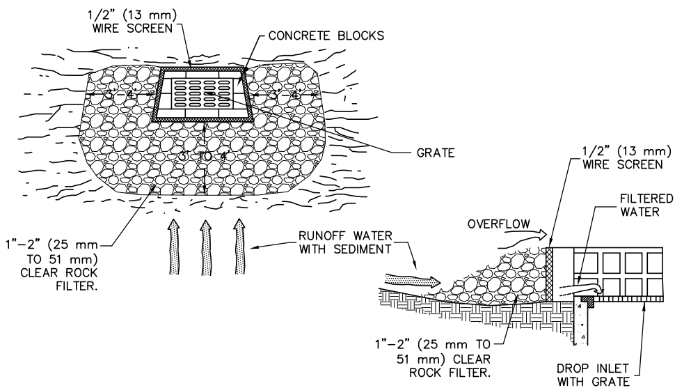
606 — BLOCK AND GRAVEL DROP INLET SEDIMENT FILTER 606 — Rock Inlet Check.dwg 5/2015
