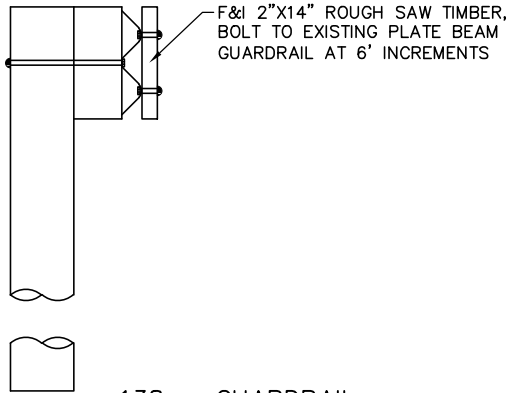
138 - GUARDRAIL OPTION 4 WOOD FASCIA 138 - Guardrail.DWG 6/2015
