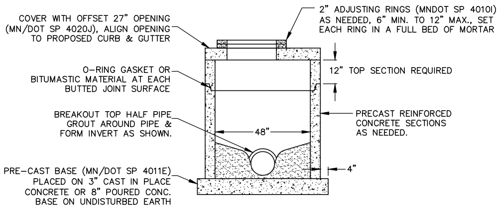
203 - STD MH (CB-MH) 203 - STD MH (CB-MH).DWG 9/2016
