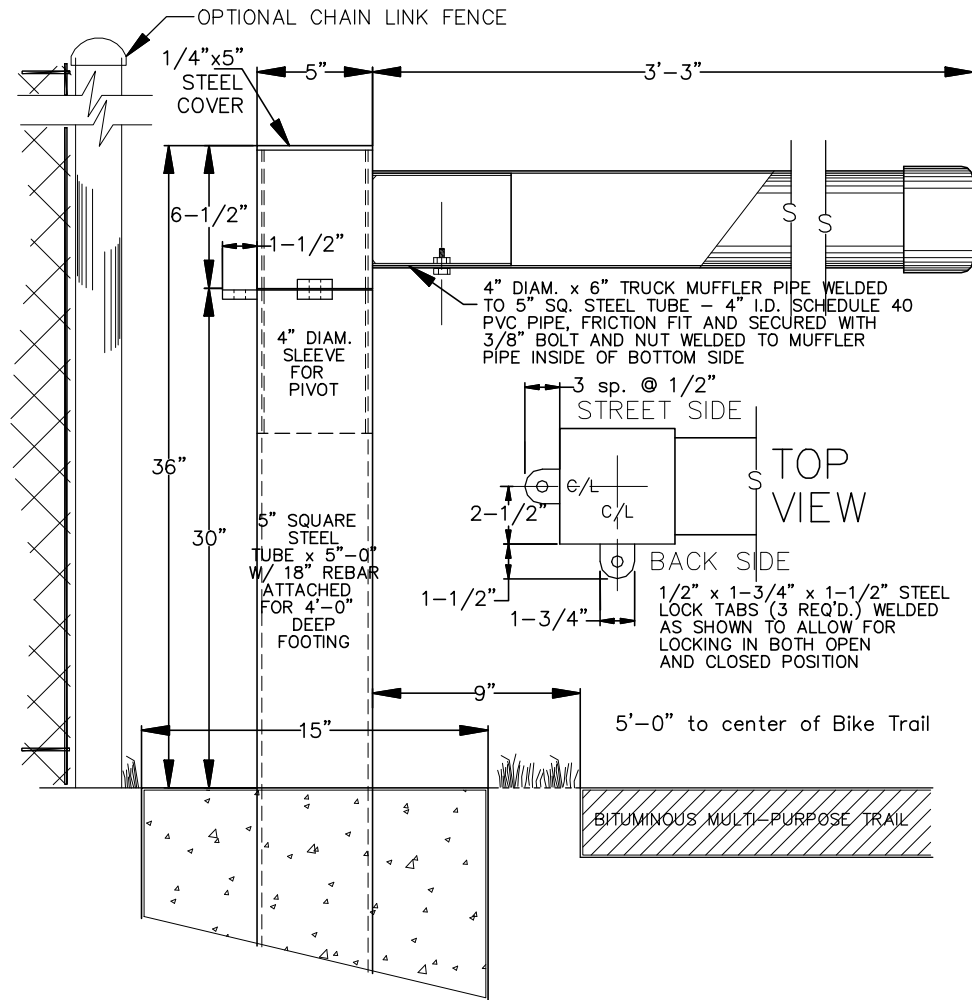
132 - VEHICLE GATE-SPECIAL 132 - Vehicular Gate (Special).dwg 6/2015
