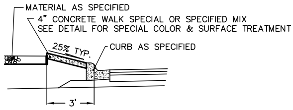
115 - 24" MAINTENANCE STRIP 115 - 4 Conc Maint. Strip.dwg 6/2015
