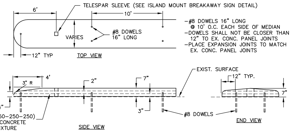
113 - 7" SURFACE CONCRETE MEDIAN 113 - 7 Conc Surf Median.dwg 9/2015
